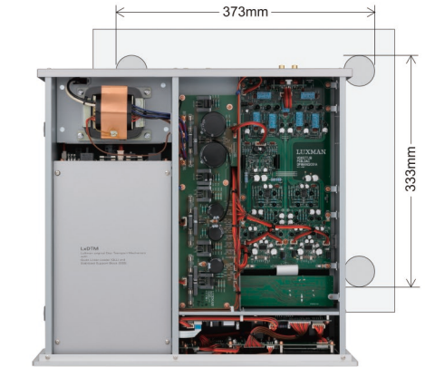
Internal configuration
