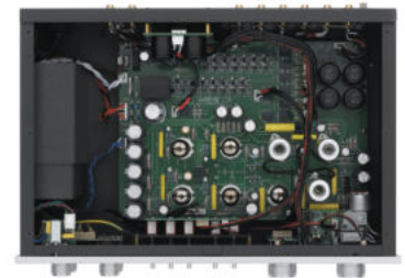
Internal configuration
